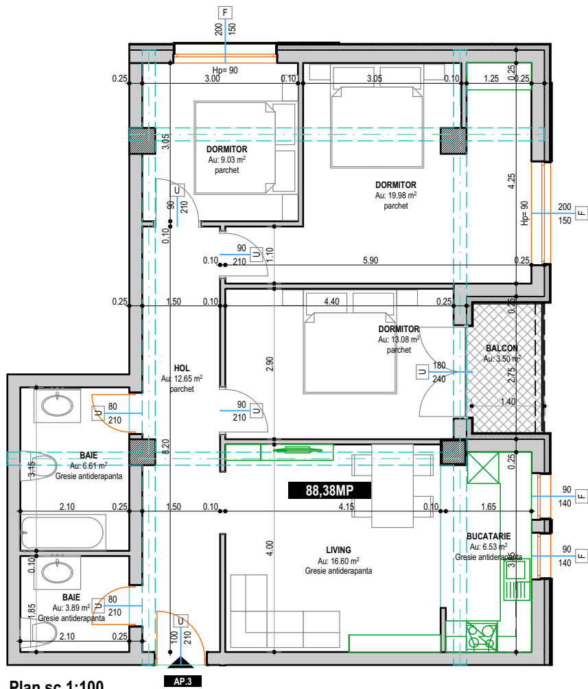
Plan sc.1:100
